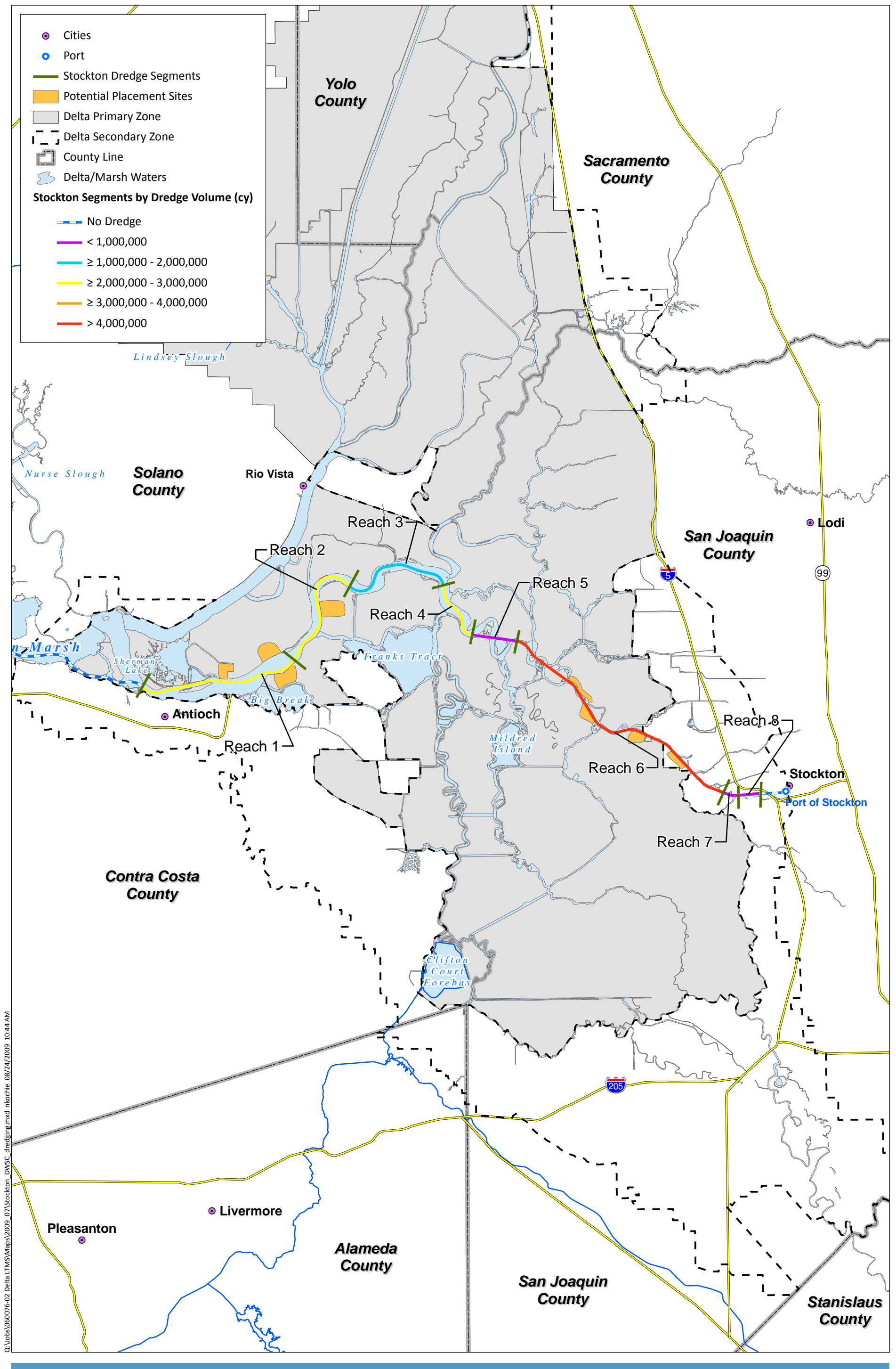
Figure 1 Stockton DWSC Potential Placement Sites, Dredging Segments, and Volumes DRAFT
